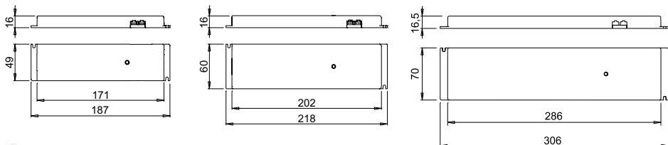
X-DRIVER 15/24D
